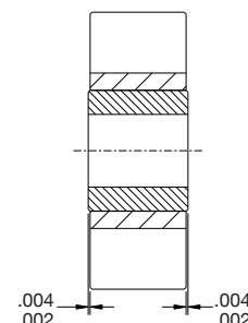
FIGURE K – IDLER BUSHING PROTRUSION
